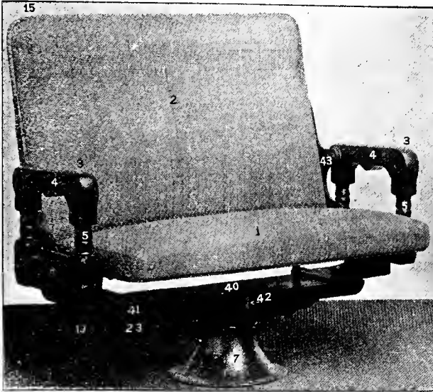
Fig. 3980. REVOLVING AND FOLDING SEAT.
